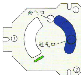
三点压紧方式 Three-point clamping drawing
